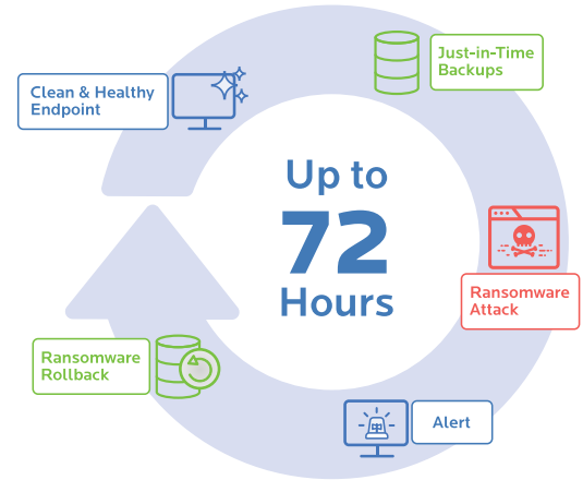
Figure 4: Ransomware Rollback
